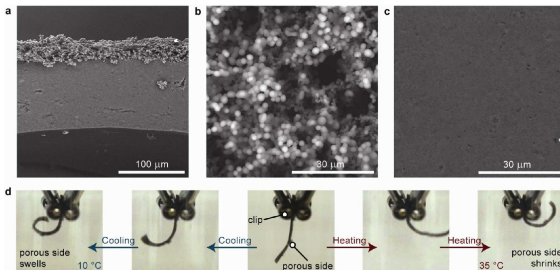
Figure 3. Microstructure and consequent behavior of ELP-rGO nanocomposite hydrogel actuators. (a) Cross-sectional SEM image showing the sharp microstructural contrast between the top and bulk of the hydrogel. (b) SEM images of the highly porous top surface and (c) relatively nonporous bottom surface. (d) Images of an anisotropic hydrogel reversibly curling in response to cooling or heating of the surrounding solution.
