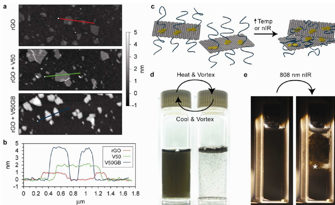
Figure 2. Effects of ELP binding to rGO. (a) AFM images ( 2 \mu\text{m} \times 5 \mu\text{m} ) of rGO sheets (top), V50-treated rGO (middle), and V50GB-treated rGO (bottom). (b) AFM height profiles from (a) show the height increase due to ELP binding. (c) Schematic of hybrid nanoparticles going from a dispersed to aggregated state in response to temperature or nIR-light due to the ITT. (d) Images of reversible temperature induced aggregation of V50GB-treated rGO. (e) Images of aggregation induced by exposure to an 808 nm nIR laser. Aggregation occurred above the laser spot site (white asterisk) due to convection.
