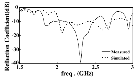
Figure 8. The result of antenna reflection coefficient.
