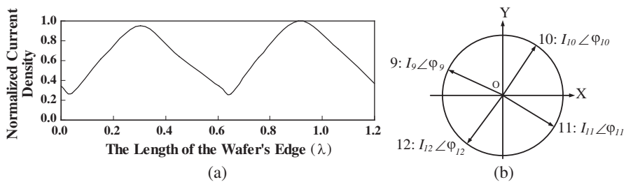
Figure 5. The simulation results concerning the amplitude and phase of the current density in the edge of the metal disk. (a) The simulated results of the amplitude of the current density in the edge of the metal disk. (b) The simulation results concerning the phase of the current density in the edge of the metal disk.
