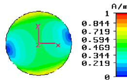
Figure 4. The distribution of the surface current density in the loaded metal disk.
