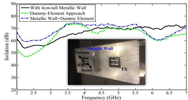
Fig. 5. Measured isolation of the proposed bistatic system with a metallic wall inserted as shown in the inset and with the dummy-element approach.
