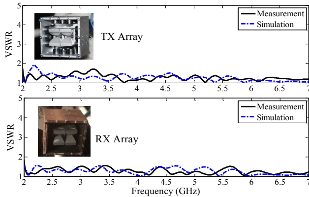
Fig. 2. Measured and simulated active VSWRs of the TX/RX Arrays shown in the inset.
