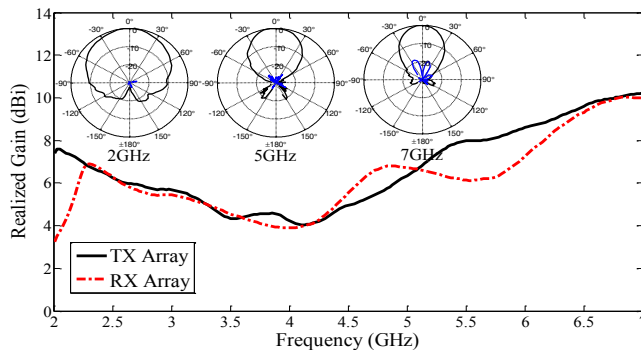
Fig. 3. Measured realized gain of TX/RX Arrays. H-plane TX radiation patterns are also shown in the inset at 2 GHz, 5GHz, and 7GHz.
