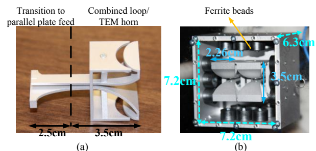
Fig. 1. (a) Geometry of the miniaturized TEM horn and (b) TX TEM horn array fully recessed inside a ferrite-loaded cavity.
