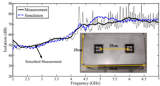
Fig. 4. Measured and simulated isolation of the proposed bistatic STAR system.
