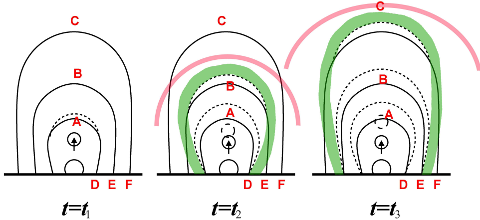
Figure 3. A schematic sketch of the formation mechanism of CME leading loops, where the CME leading loop ( green ) are apparently-moving density enhanced structure that is generated by the successive stretching of magnetic field lines as the erupting core structure, e.g., a flux rope, continues to push the overlying field lines to expand outward successively. The piston-driven shock is shown as pink lines (from Chen 2009a).
