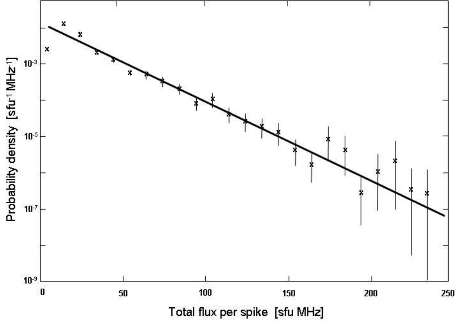
Figure 9. Distribution of total flux (flux density integrated in frequency) of narrowband spikes. The line is an exponential fit which is given in Equation (??).
