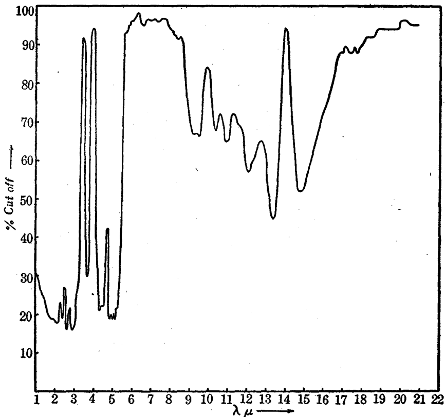
FIG. 3. Infra-red absorption spectrum of calcite (Specimen II).
