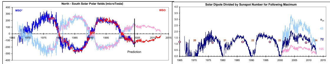
Figure 10: (Left) The axial magnetic ‘dipole moment’ of the Sun, defined as the difference between the (signed) magnetic field strength near the North Pole and near the South Pole, for the past four solar cycles. To facilitate comparison of cycles, a ‘ghost’ mirror image is also plotted. Data from Mount Wilson Observatory (blue) has been scaled to match observations from Wilcox Solar Observatory (red). (Right) The polar field variation at the left scaled by the maximum smoothed sunspot number for the next cycle suggesting the same variation for each cycle, i.e. that the cycle maximum is controlled by the polar fields at the preceding minimum. For Cycle 24, the maximum was not known, but a very high value (165) or a very low value (45) does not fit the pattern. A maximum size of 72 for Cycle 24 seems to be the just right ‘Goldilocks’ value.
