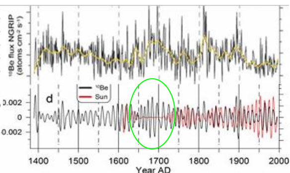
Figure 9: (Top) ^{10}\text{Be} flux from the NGRIP ice core (Greenland). (Bottom) The ^{10}\text{Be} data band pass filtered at 8–16 years [Berggren et al., 2009]. The red curve is the filtered GSN series.
