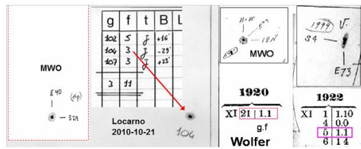
Figure 2: (Left) Part of a drawing made at Locarno, showing that the spot with penumbra designated 104 was counted three times (weight 3); the insert shows the same spot from Mt. Wilson. (Right) Two spots with the same area on drawings from Mt. Wilson and counted with weight 1 by Wolf, in each case as one group with one spot (Wolf’s notation: groups.spots = 1.1 ), as the group was the only group on the disk
