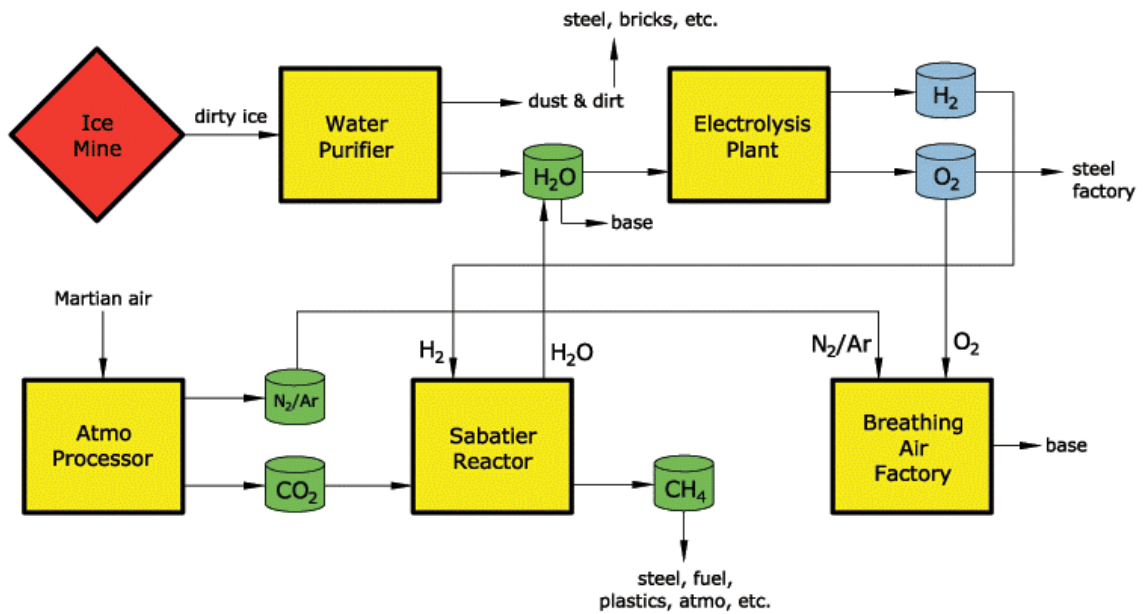
Figure 2. Marsbase Materials Flow
